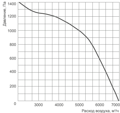
SDT 70-40/35.2D-3
