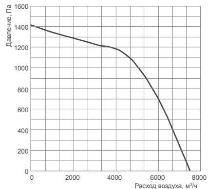
SDT 80-50/35.2D-3
