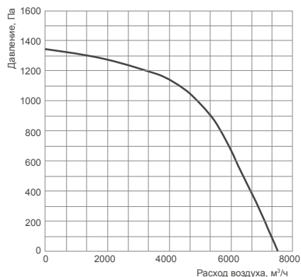
SDT 90-50/35.2D-3
