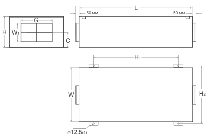
Energy W 4000/6000
