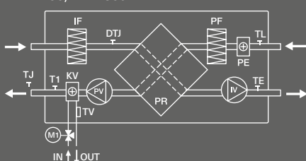
HPW 450, HPW 800
