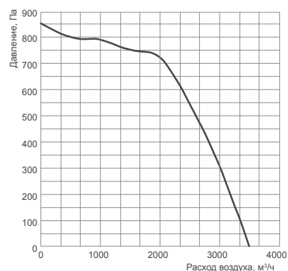
SDT 70-40/35.2D-3
