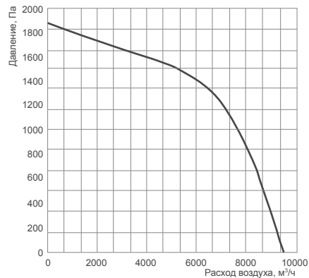
SDT 100-50/40.2D-4
