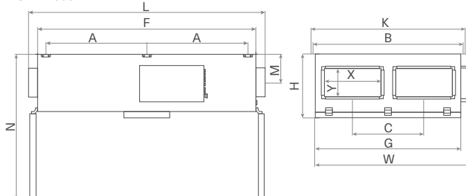
CPW 1500
