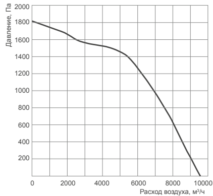
SDT 90-50/40.2D-4
